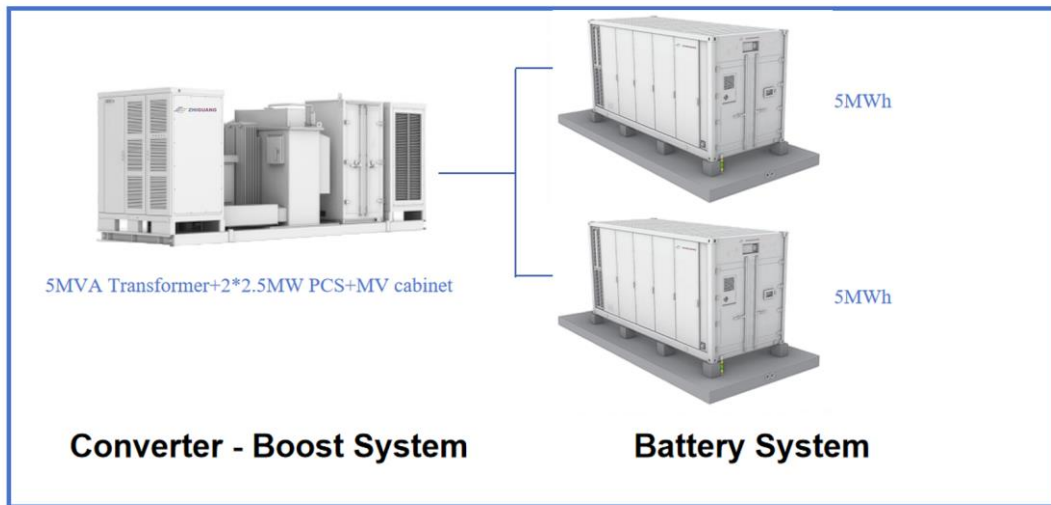
5MW/10MWh BESS Diagram
