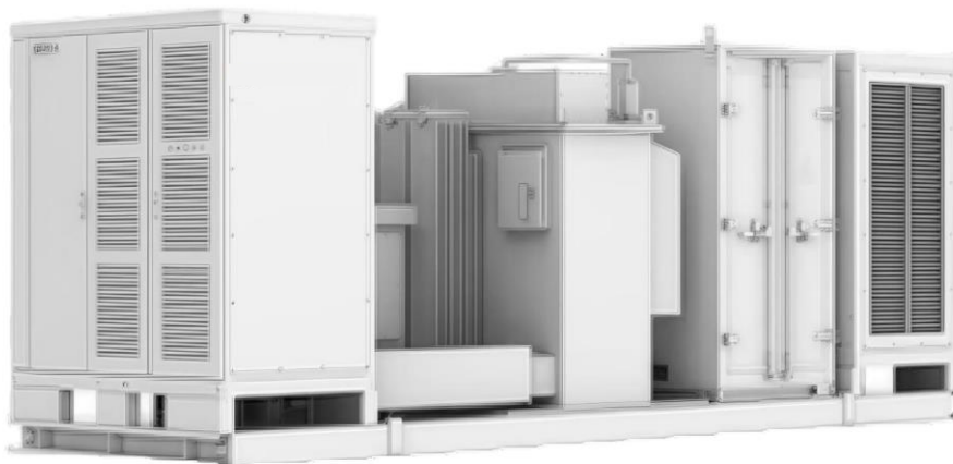
5MVA Transformer+2*2.5MW PCS+MV cabinet
