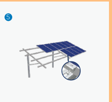
Fix the solar module with Inter Clamp Kit & End Clamp Kit
